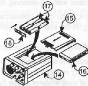
Figure 6 - Installing the Batteries
